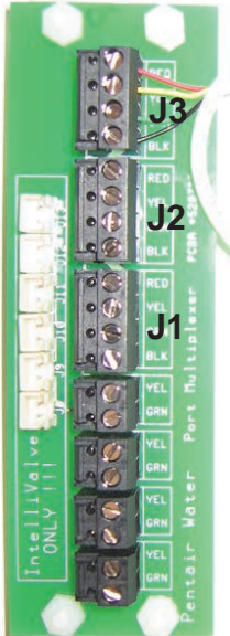
Expansion Board
